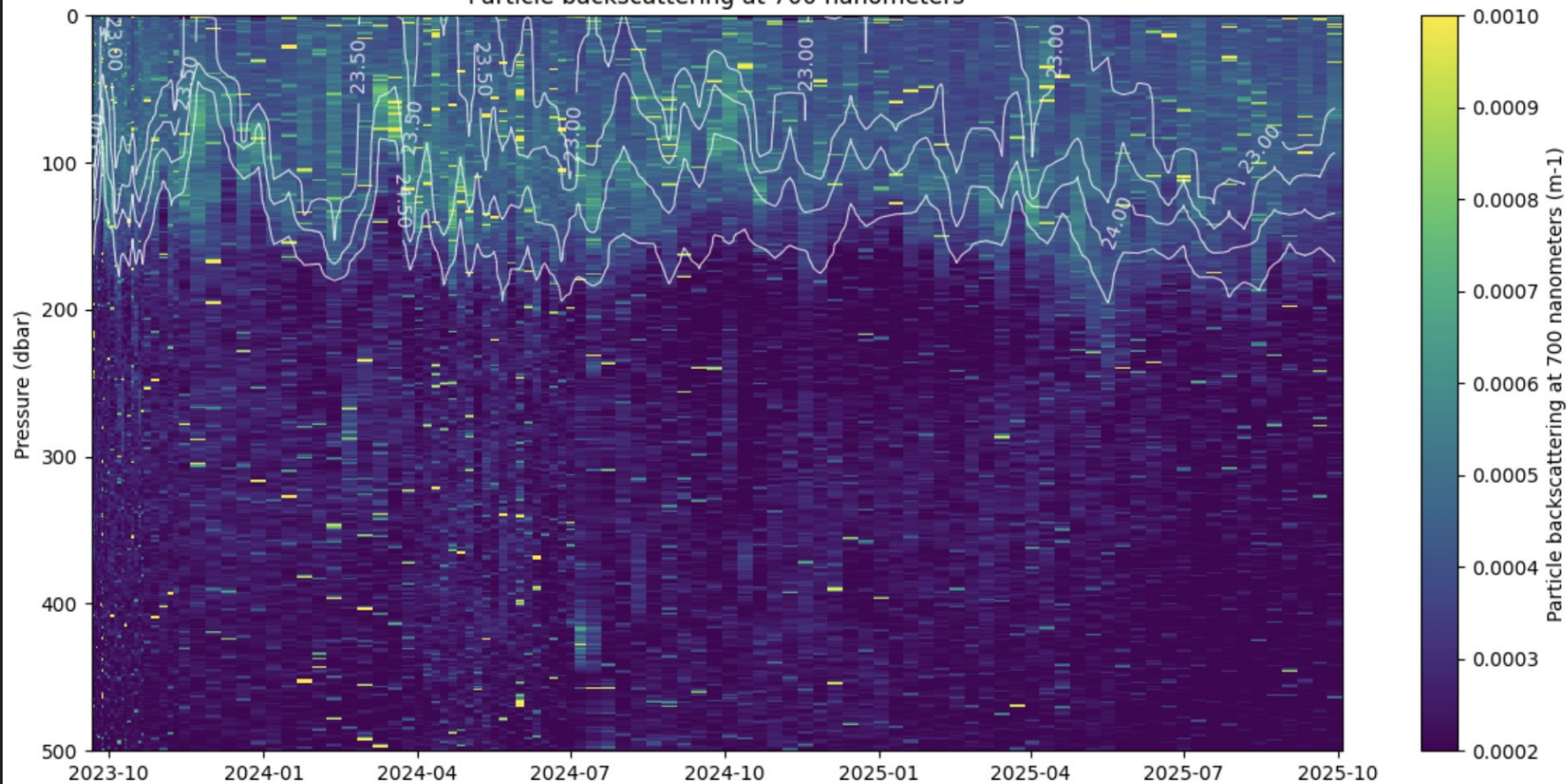
Particle backscattering at 700 nanometers
