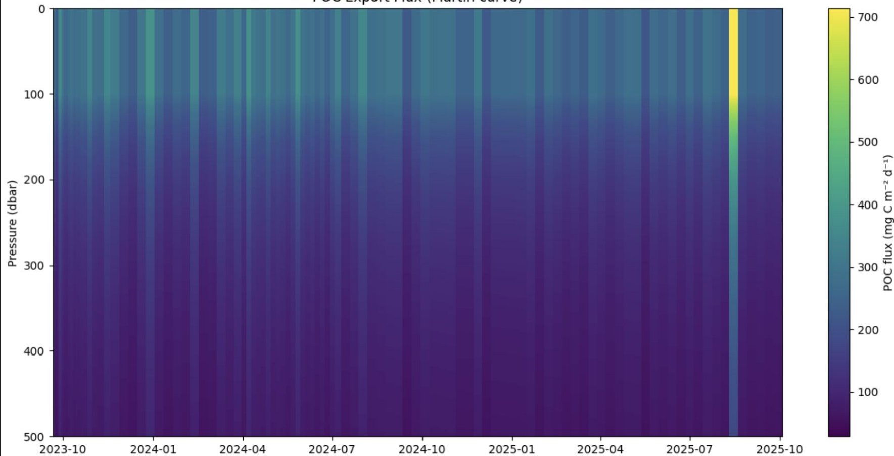
POC Export Flux (Martin curve)
